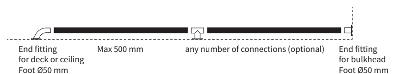
Mounting with bolt or screw from outside
